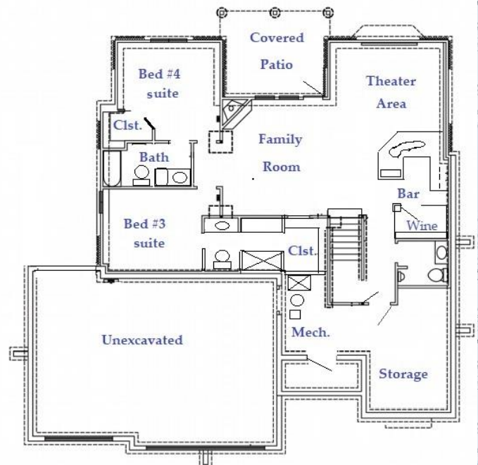
LL - approx. 1,440 sq. ft.
