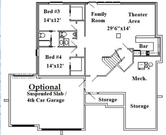
Lower Level: approx. 1,384 sq. ft.
