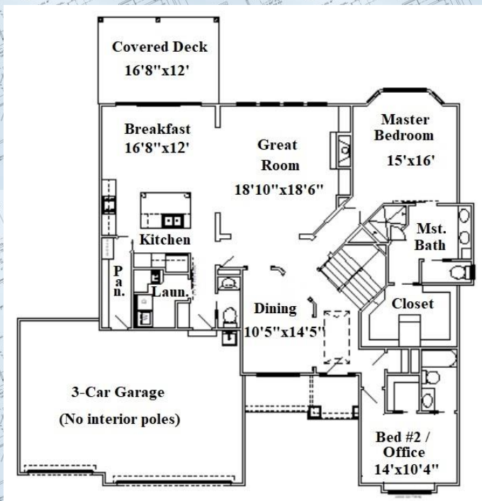
Main Level: approx. 2,051 sq. ft.
